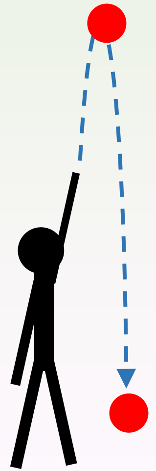
vertical throw
