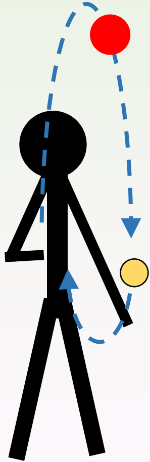
juggling
